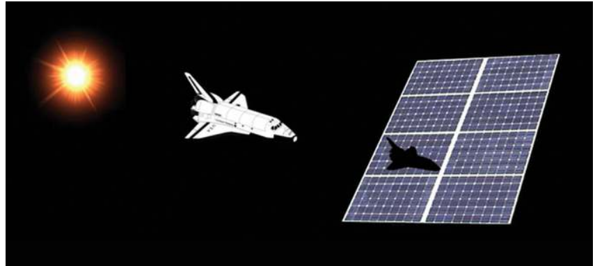
Figure 9. Cells in shadow produce no current, limiting total power available from an array
