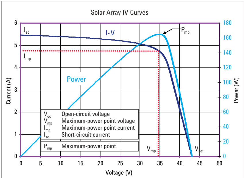
Figure 3. Four variables determine the I-V and power curves that can be used to approximate solar-cell output
