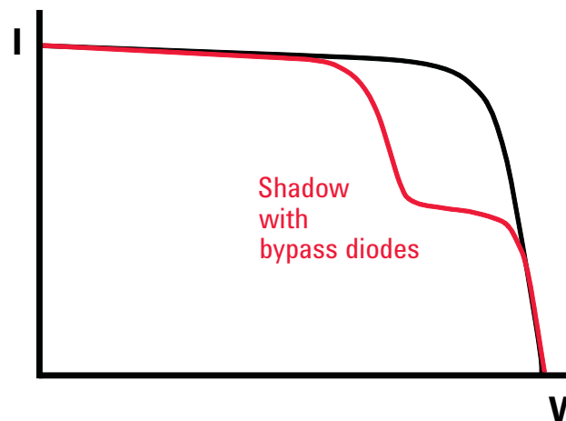
Figure 11. Some solar array simulators are capable of mimicking solar arrays in shadow
