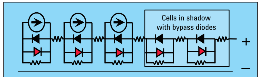
Figure 10. Adding bypass diodes to the cell design will improve performance when the array is in shadow
