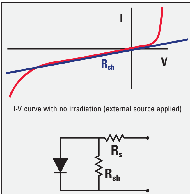
Figure 2. I-V curve and equivalent circuit for photovoltaic cell in shadow
