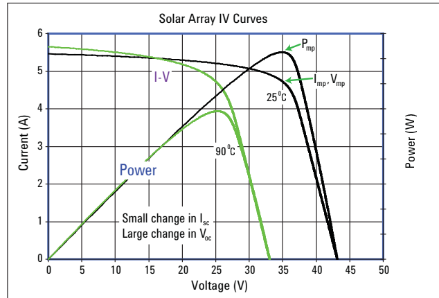
Figure 5. Temperature variation has a strong effect on output power
