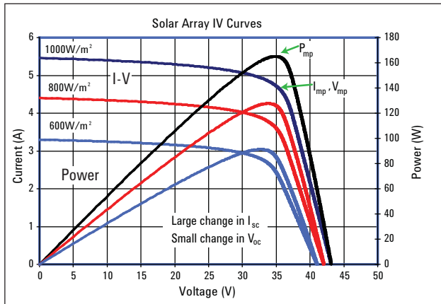
Figure 4. A solar array's I-V and power curves vary with irradiation level
