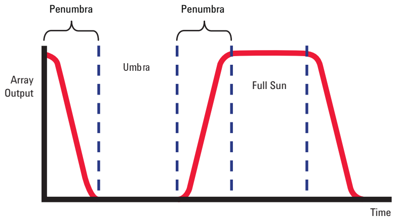
Figure 8. Available output power varies as the satellite enters, transits, and exits darkness and then re-enters full-sun condition
