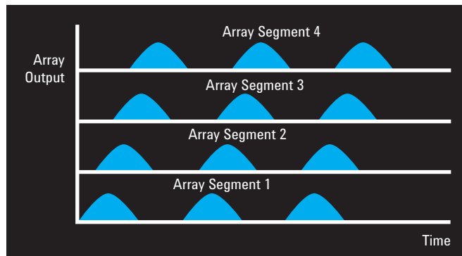
Figure 7. Available output power from each panel rises and falls as the satellite spins
