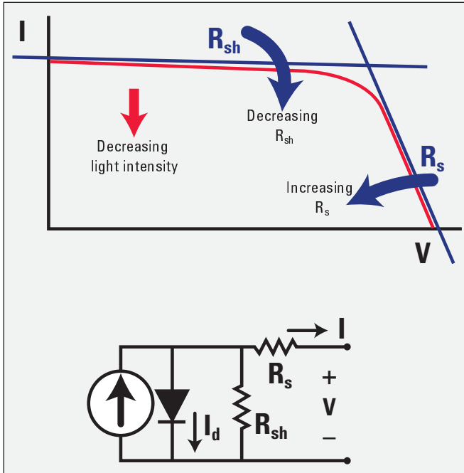
Figure 1. I-V curve and equivalent circuit for illuminated photovoltaic cell
